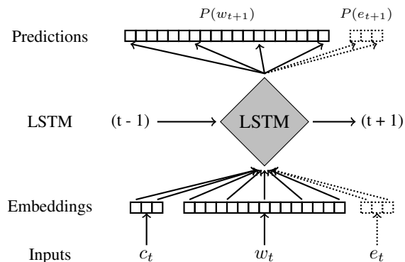
Figure 1: LSTM Script System at timestep t .
